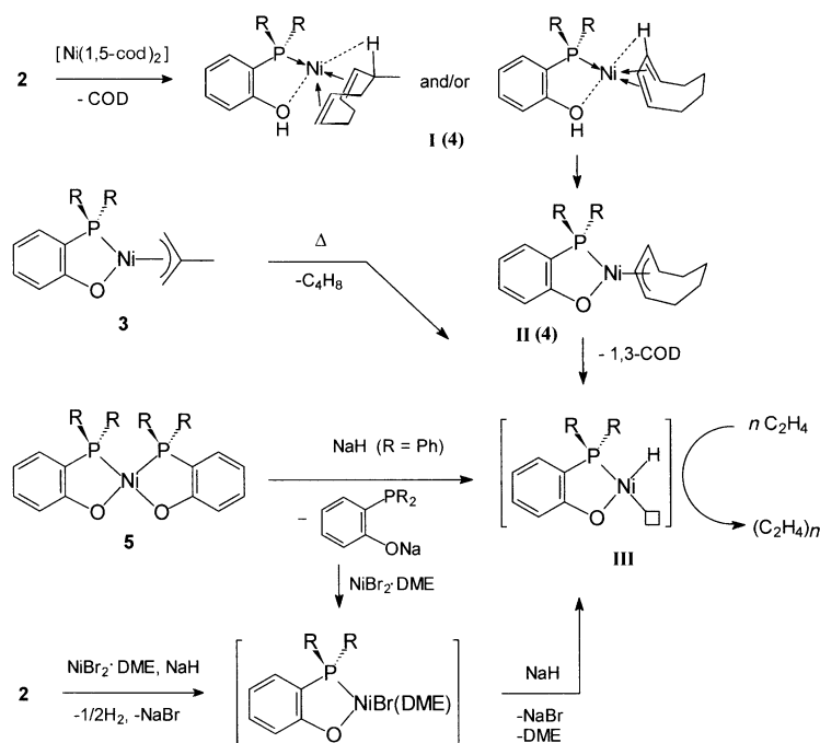
Scheme 3. Proposed formation of 2-phosphanilphenolonickel hydride catalysts.
