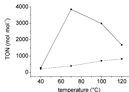
Figure 2. Temperature dependence of the TON for the polymerization of ethylene with 4 PPHH in toluene, a) p_{\text{start}} = 30 \text{ bar} , C 2 H 4 150–200 mmol, 4 PPHH 0.24 mmol (dash), b) p_{\text{start}} = 50 \text{ bar} , C 2 H 4 460–480 mmol, 4 PPHH 0.1 mmol (solid).
