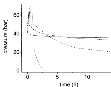
Figure 4. Pressure–time plots for the polymerization of ethylene with \mathbf{4}_{\text{PPHH}} (solid), \mathbf{4}_{\text{CCHH}} (dash dot), \mathbf{4}_{\text{IBBB}} (dash) and \mathbf{4}_{\text{PPOH}} (dot); bath temperature 100 °C.
