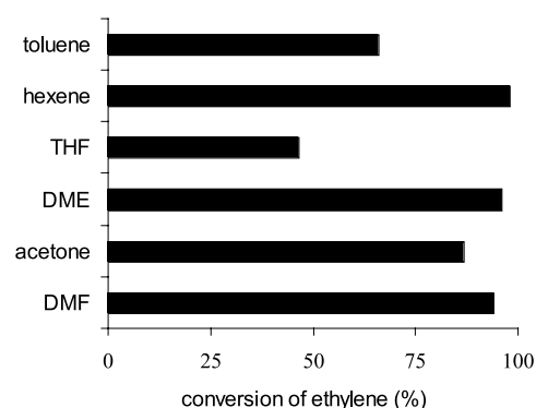
Figure 5. Polymerization of ethylene with 4 PPHH in various solvents (conditions: \text{C}_2\text{H}_4 0.4–0.6 mol, p_{\text{start}} 50 bar, 4 PPHH 0.1 mmol, 100 °C).
